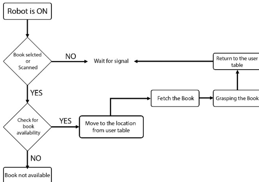
Figure 6.1 Program flow
