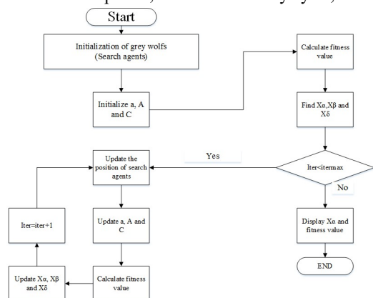
Fig 7 GWO Algorithm for MPPT
