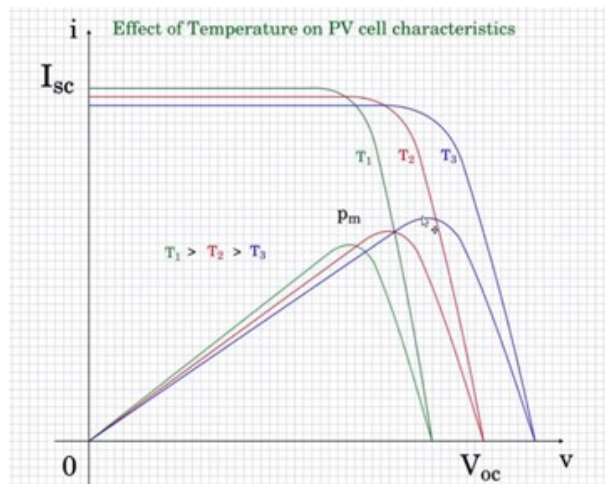
Fig.2. Solar I-V Characteristic with changing temperature along with solar output power.
