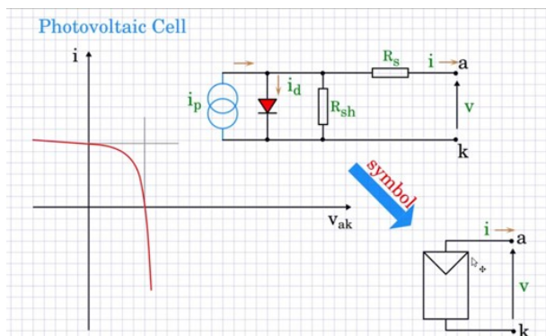
Fig.1. Practical solar cell.
