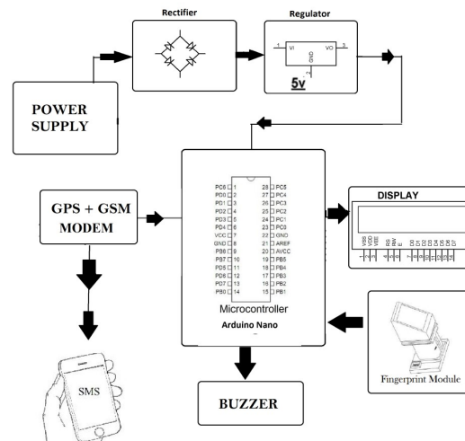
Block diagram of the proposed system
